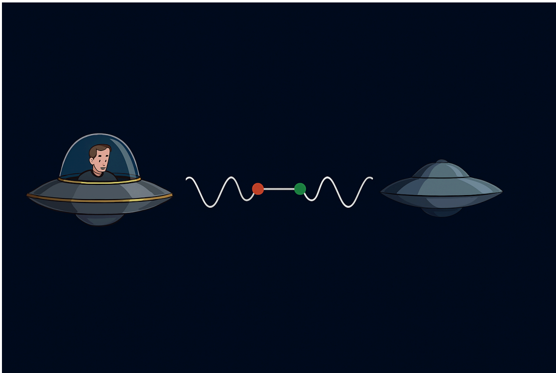
Figure 2: Relativistic symmetry between two spacecraft
