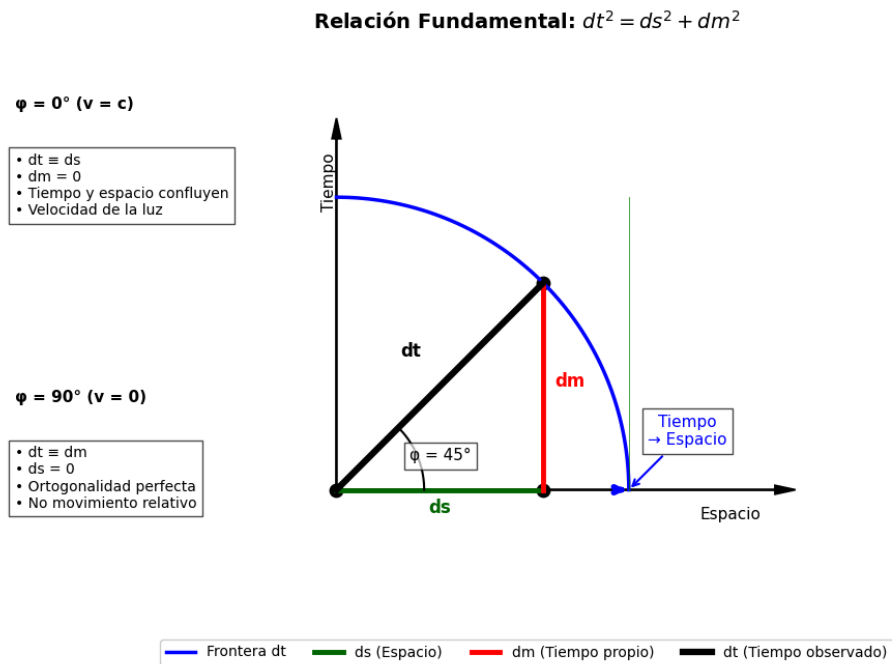
Figure 1: space-time
